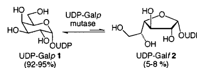
Figure 1. UDP-Galp mutase catalyzes the interconversion of UDP-Galp ( 1 ) and UDP-Galf ( 2 ). The pyranose isomer 1 is favored.
