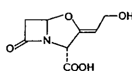
Clavulanic acid ( 2 )
