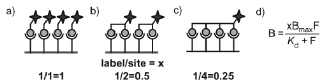
Figure 1. End-labeled materials can be used to reveal multivalent interactions. The number of labels bound depends on the number of binding sites occupied per multivalent ligand (parts a–c). The binding of end-labeled multivalent ligands at saturation ( B_{\max} ) will vary according to valency (equation shown in part 1d, B is moles of bound ligand, F is the free multivalent ligand concentration).
